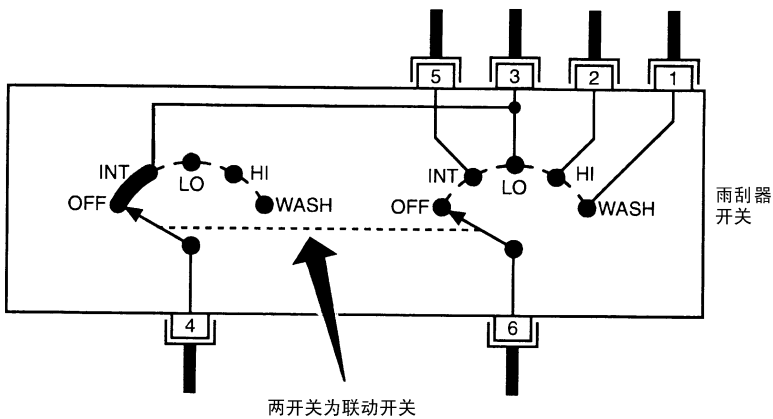
(开关图)
