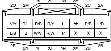
G1-13 EVAPORATOR TEMPERATURE SENSOR (I) 蒸发器温度传感器 (I)
