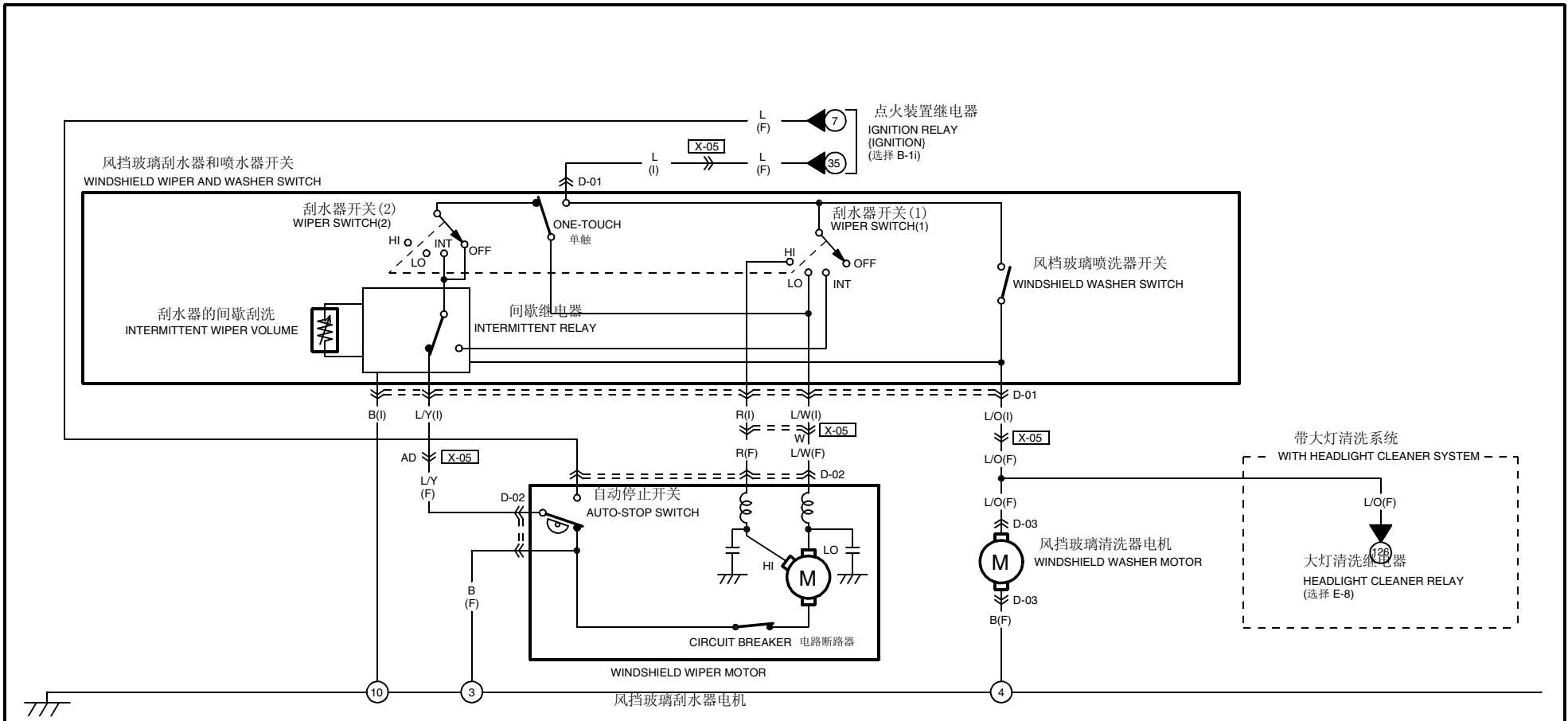
D-01 WINDSHIELD WIPER AND WASHER SWITCH (I)
