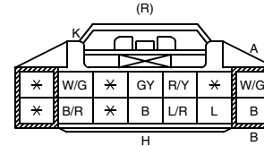
K2-05 REAR (R) SHORT CORD WITH POWER SEAT FRONT BUCKLE SWITCH LH (R) — WITHOUT POWER SEAT 左侧前带扣开关——不带电动座椅 (短索)
