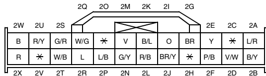
K2-07 LOCK RELEASE SOLENOID LH (DR3) 左侧解锁电磁阀
