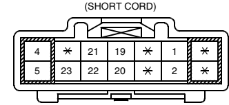
K2-05 REAR (R) SHORT CORD WITH POWER SEAT FRONT BUCKLE SWITCH LH (R) — WITHOUT POWER SEAT 左侧前带扣开关——不带电动座椅 (短索)
