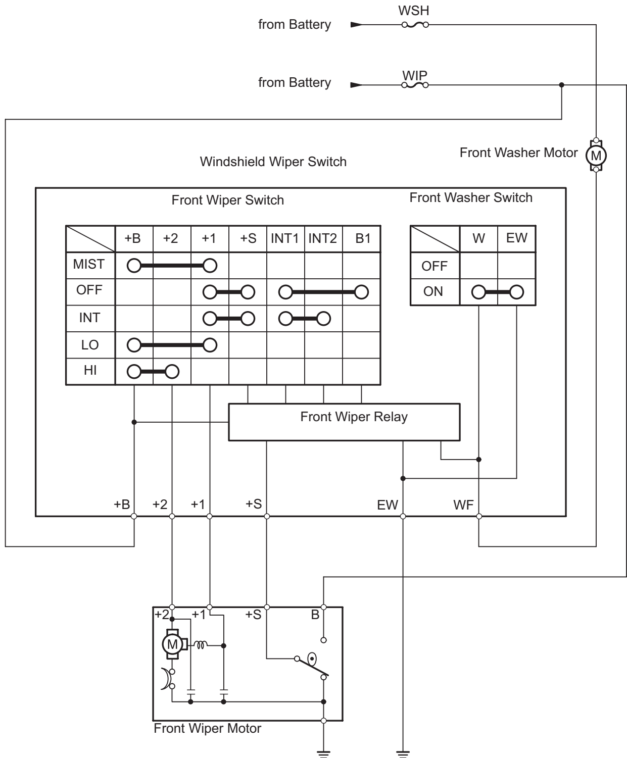
Front Wiper and Washer System
